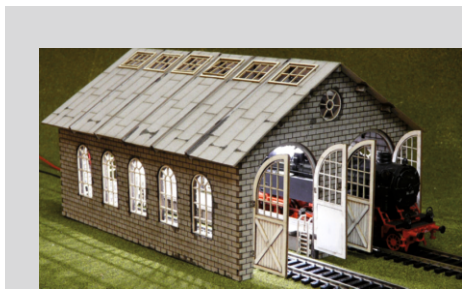
LS-009 - Double Engine Loco Shed HO/OO 192 X 136 X 110 mm
